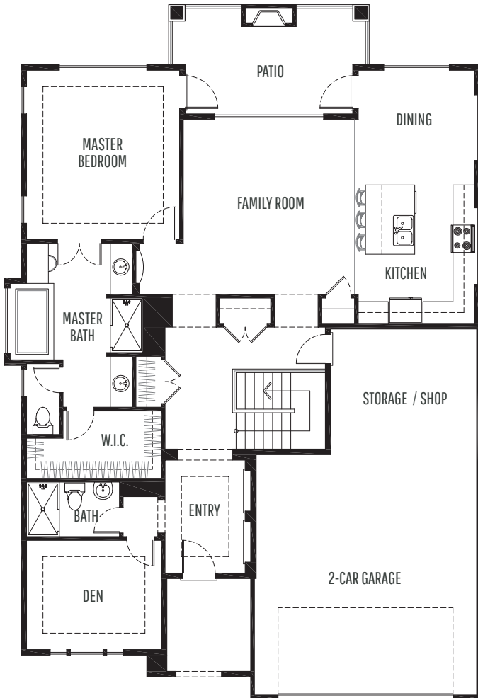
MAIN LEVEL
