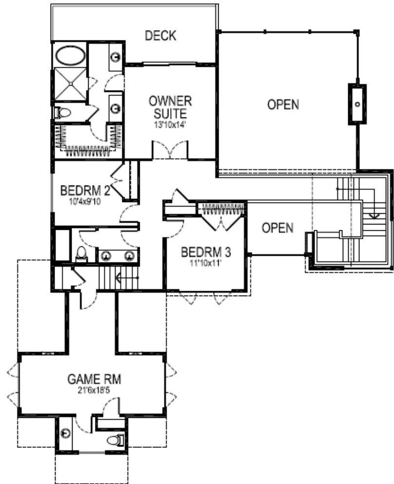
UPPER LEVEL
